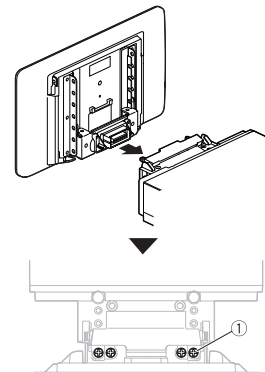
① Vite a testa bombata (4 mm × 6 mm)
